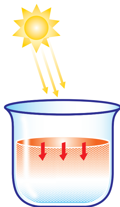
Radiation
