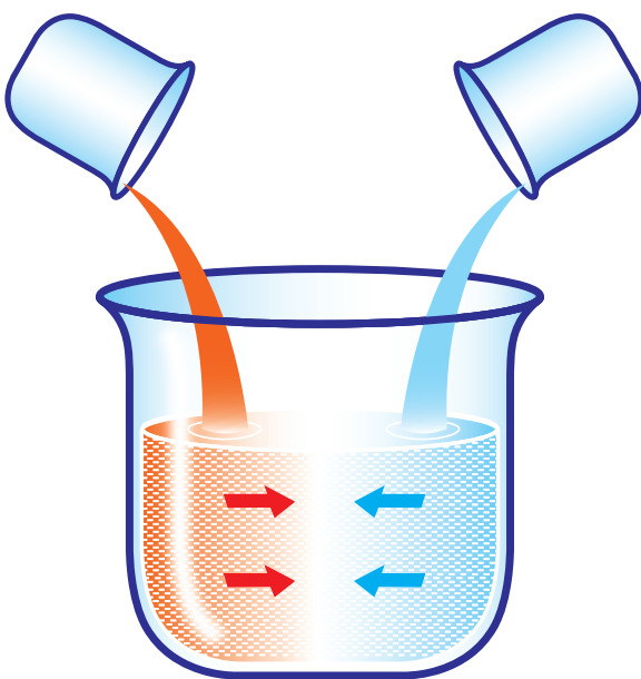
Convection
