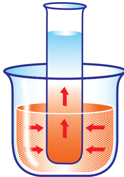
Conduction
